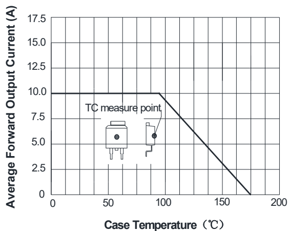
FIG1: I_o - T_c Curve
